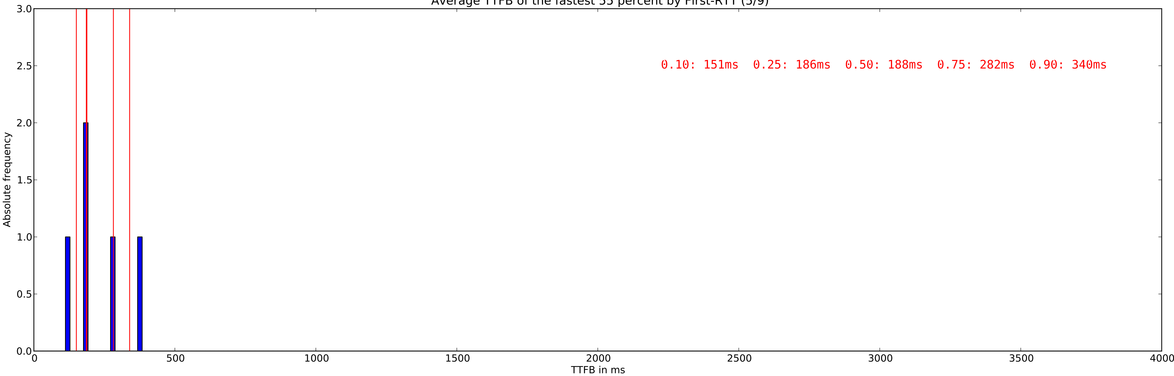
Average TTFB of the fastest 55 percent by First-RTT (5/9)
