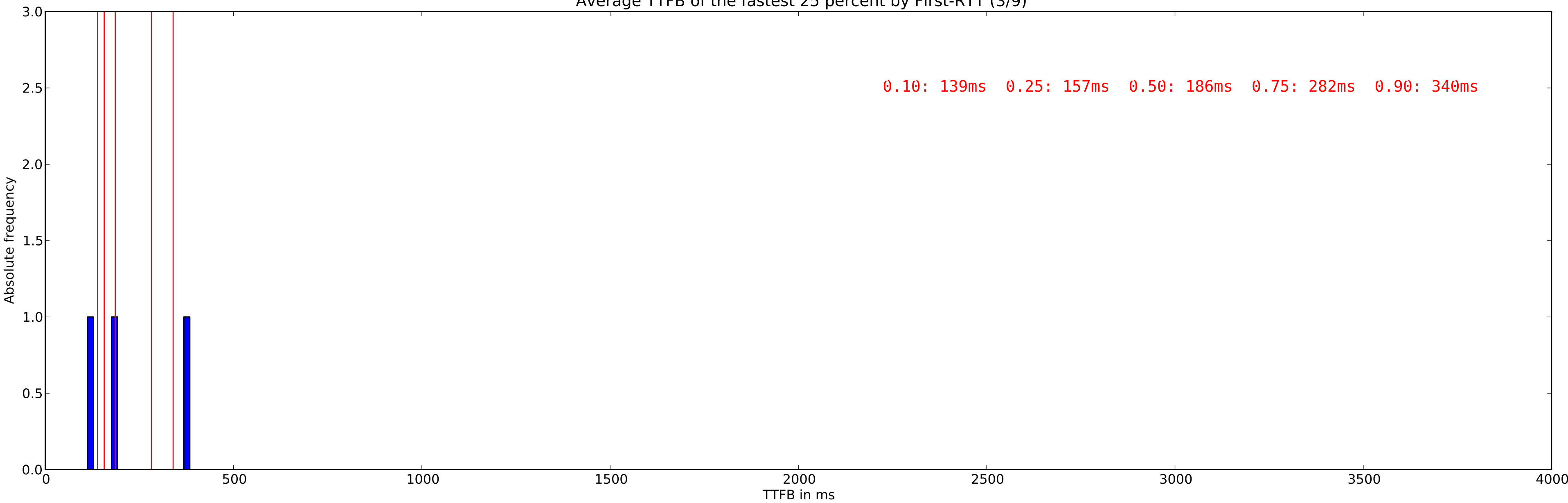
Average TTFB of the fastest 25 percent by First-RTT (3/9)
